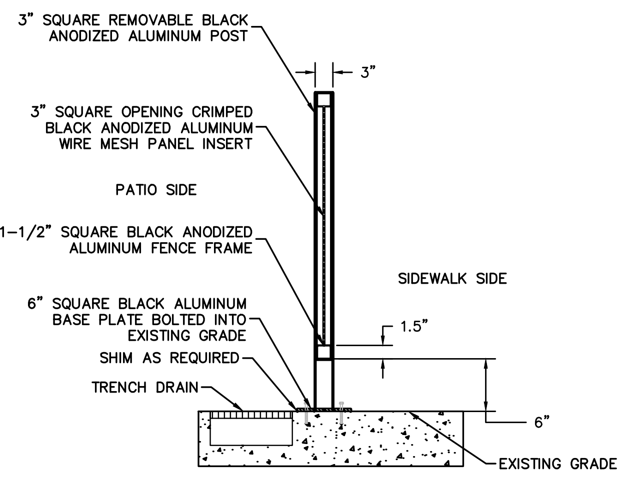
SECTION AT REMOVABLE RAILING PANEL NOT TO SCALE
