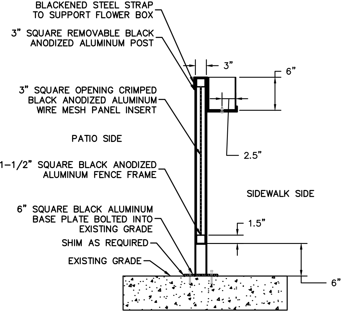
SECTION AT REMOVABLE RAILING PANEL NOT TO SCALE
