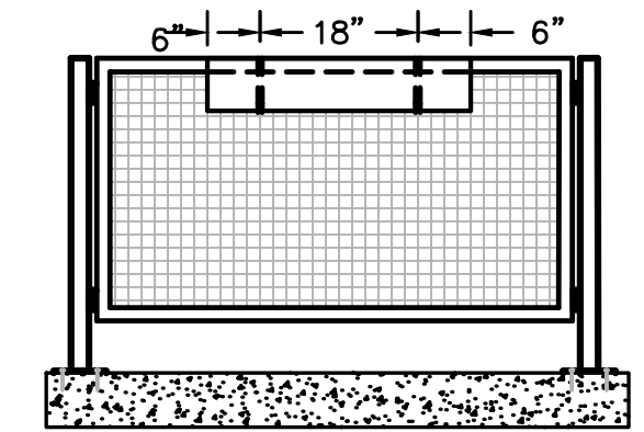
ELEVATION AT REMOVABLE RAILING PANEL NOT TO SCALE
