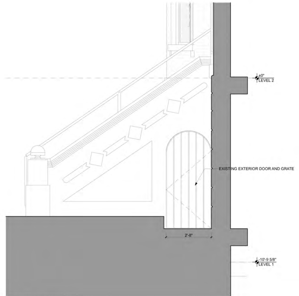
4 EXISTING FRONT STAIR SECTION SCALE: 1/2" = 1'-0"
