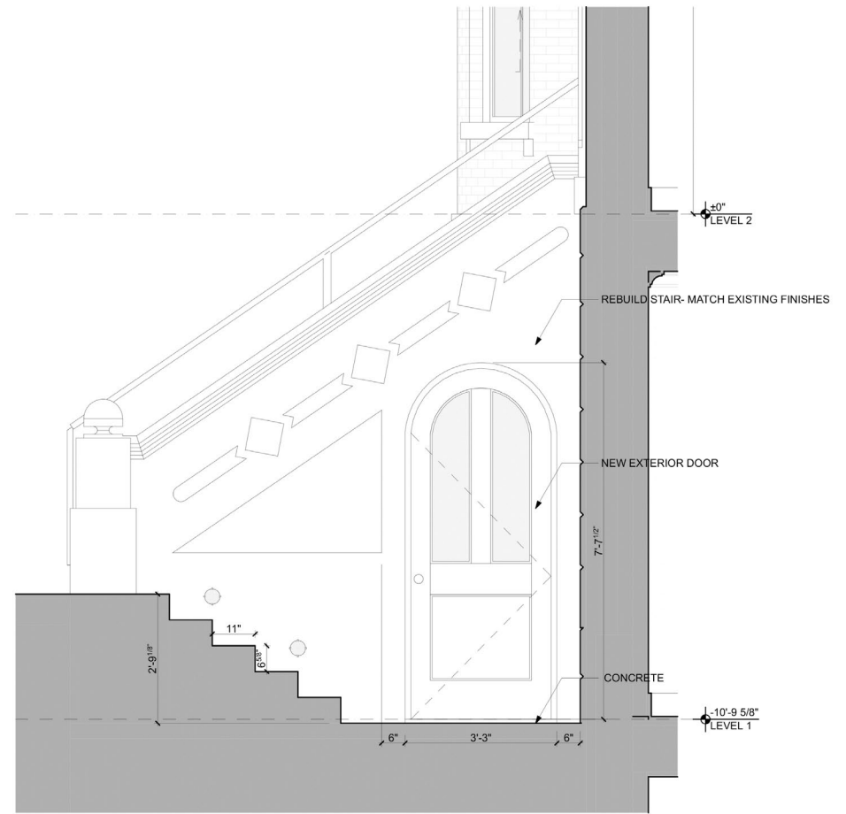
2 PROPOSED FRONT STAIR SECTION SCALE: 1/2" = 1'-0"
