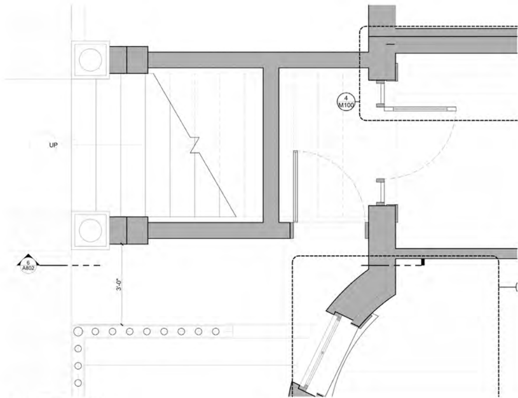
3 EXISTING FRONT STAIR PLAN SCALE: 1/2" = 1'-0"
