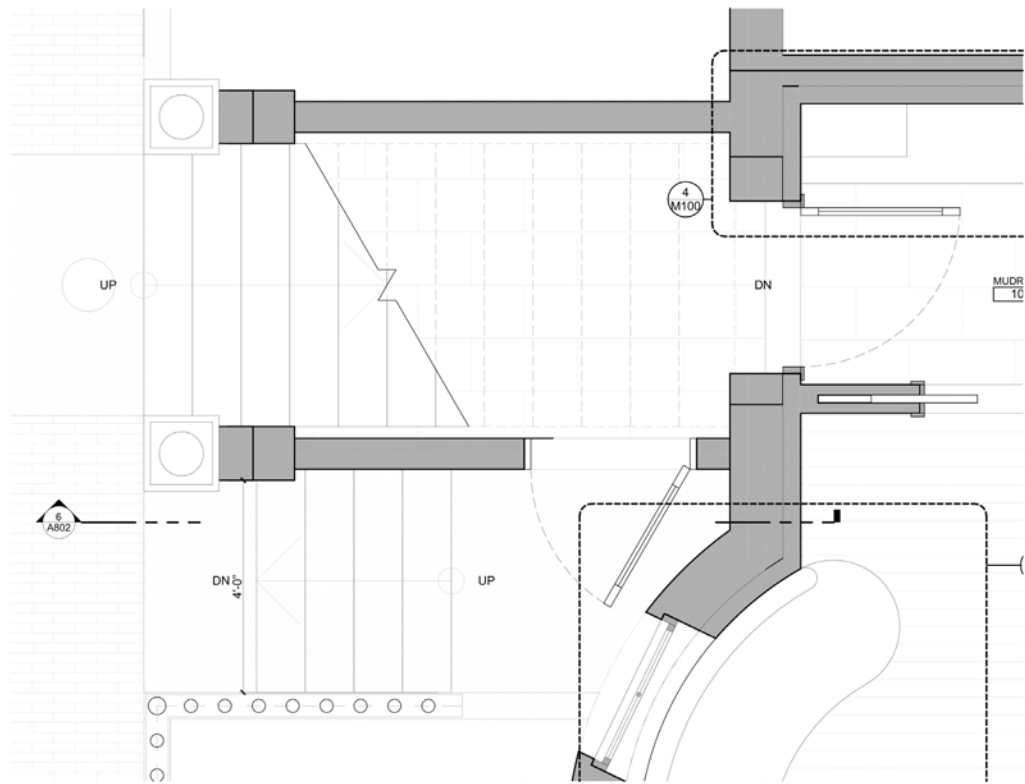
1 PROPOSED FRONT STAIR PLAN SCALE: 1/2" = 1'-0"
