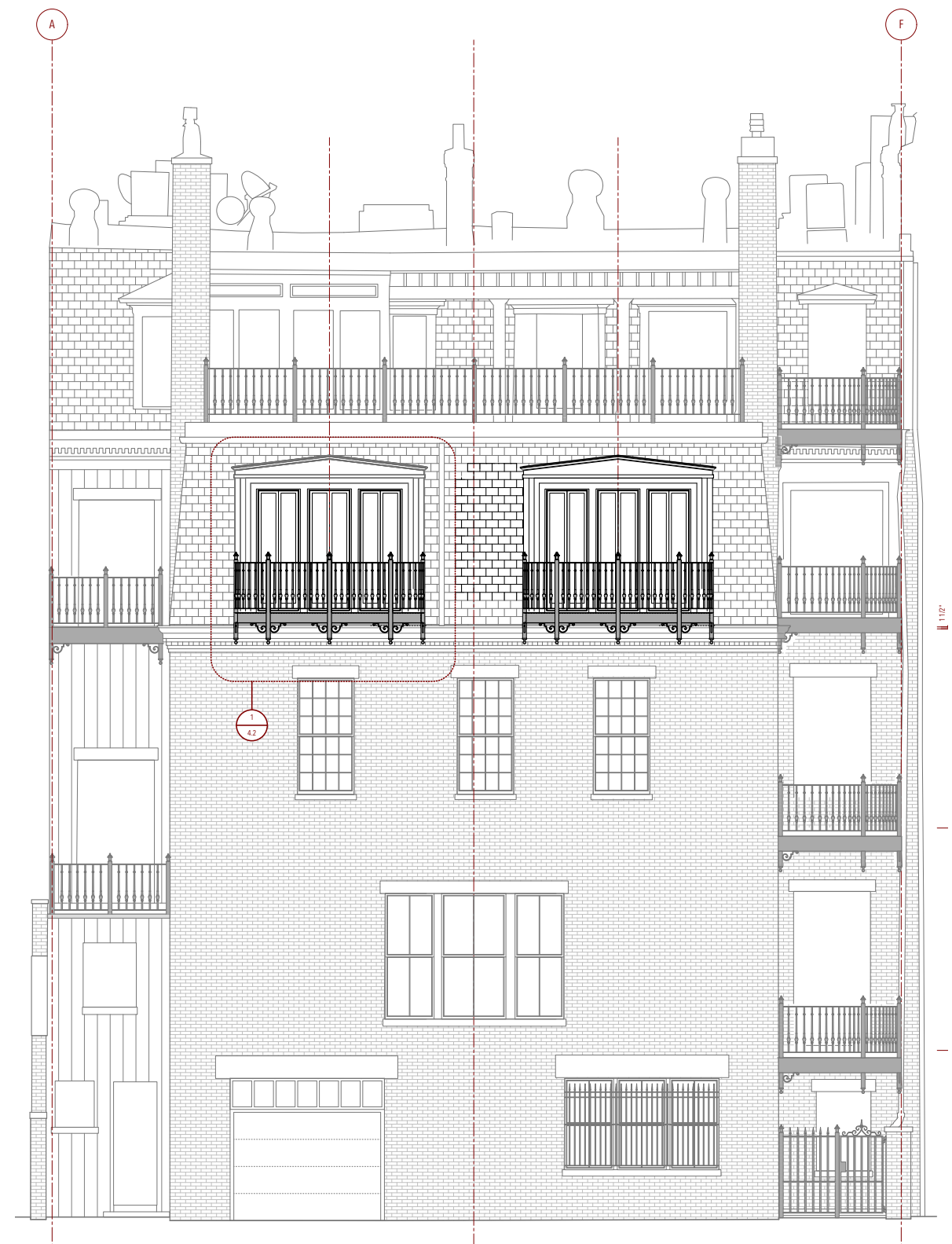
PROPOSED ELEVATION
