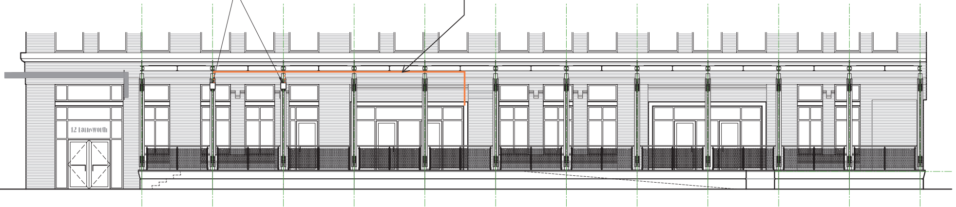
ELEVATION VIEW - FARNSWORTH STREET
