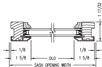
Horizontal Section
