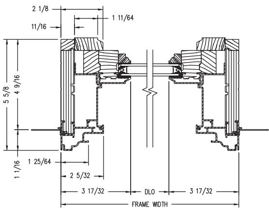
Horizontal Section
