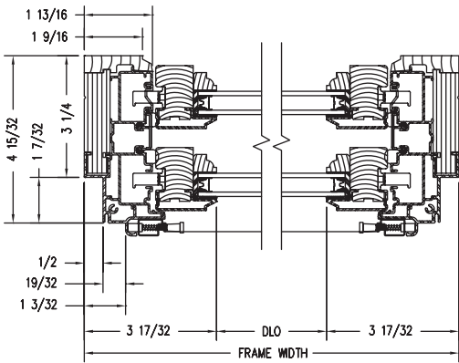
Horizontal Section
