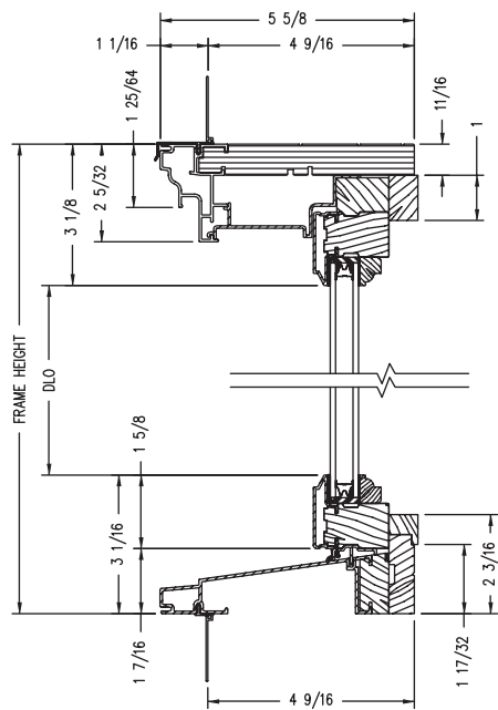
Vertical Section
