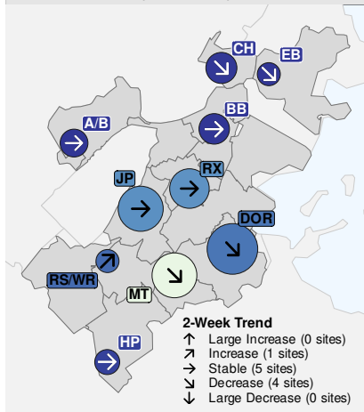
COVID-19 Wastewater Levels & Trends (16-Mar-2025)
