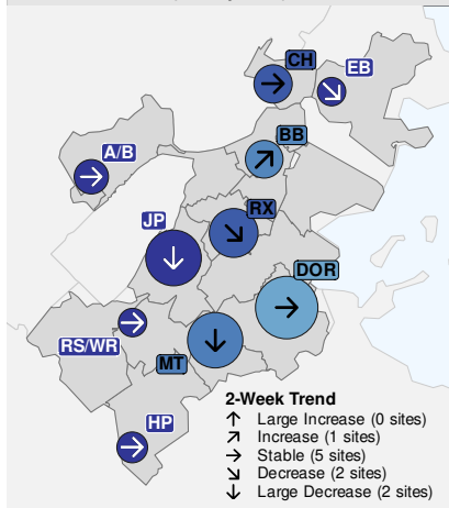
COVID-19 Wastewater Levels & Trends (04-May-2025)
