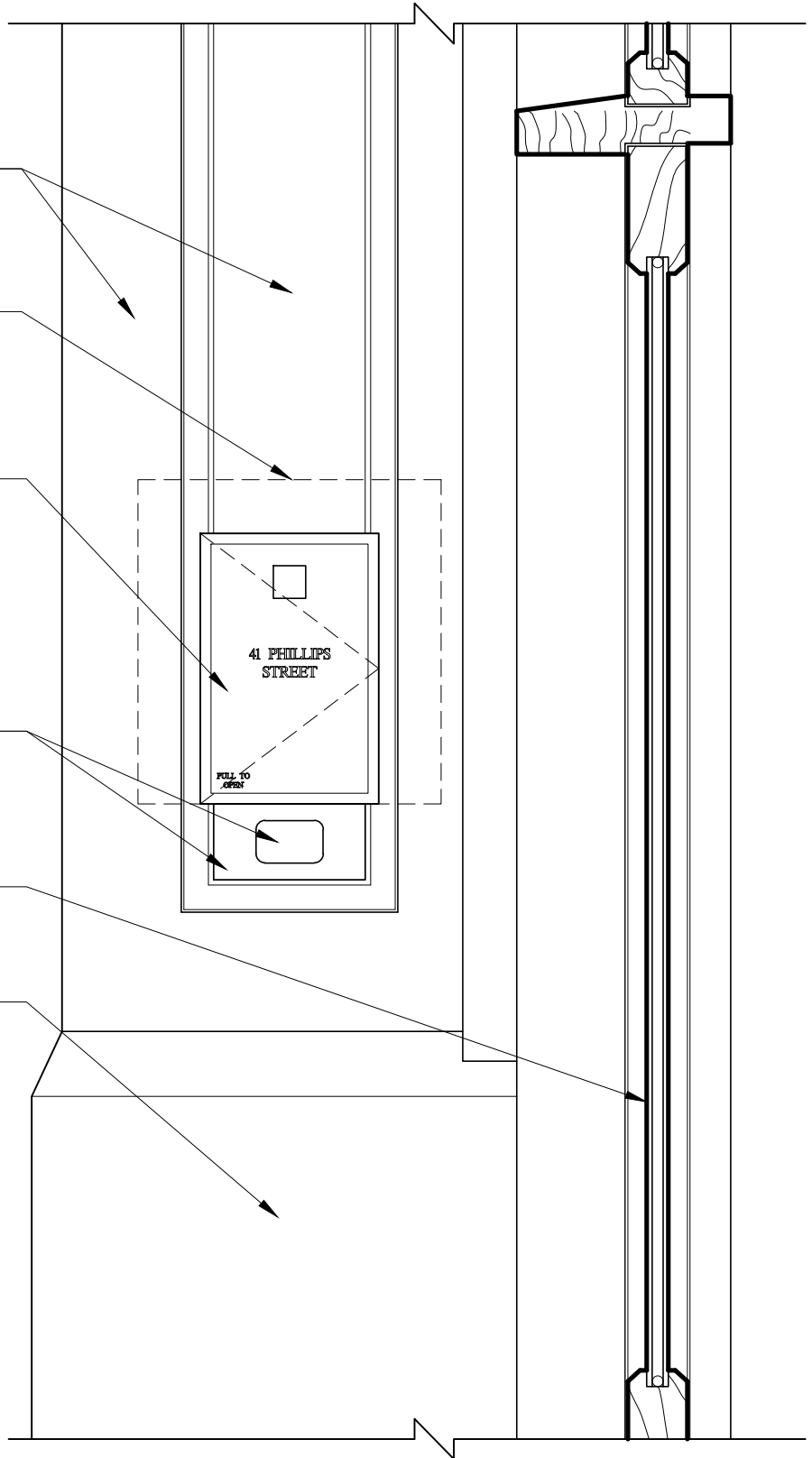
1 PARTIAL ELEVATION @ BUILDING ENTRY DOOR JAMB
