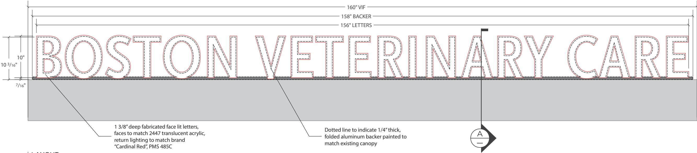
01 | LAYOUT 1" = 1'-0"
