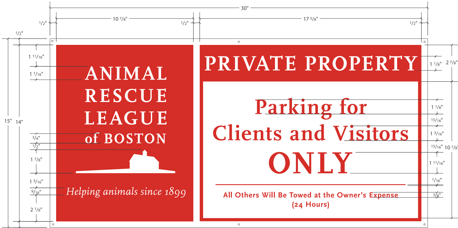
01 | GRAPHIC LAYOUT 3" = 1'-0"
