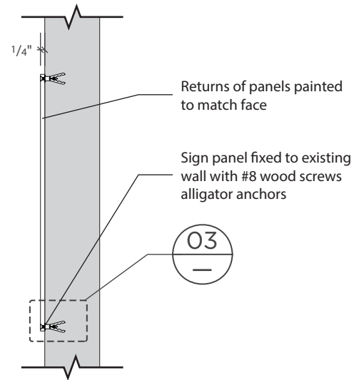
02 SIDE VIEW 1 1/2" = 1'-0"
