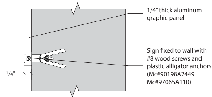
03 MOUNTING DETAIL 6" = 1'-0"
