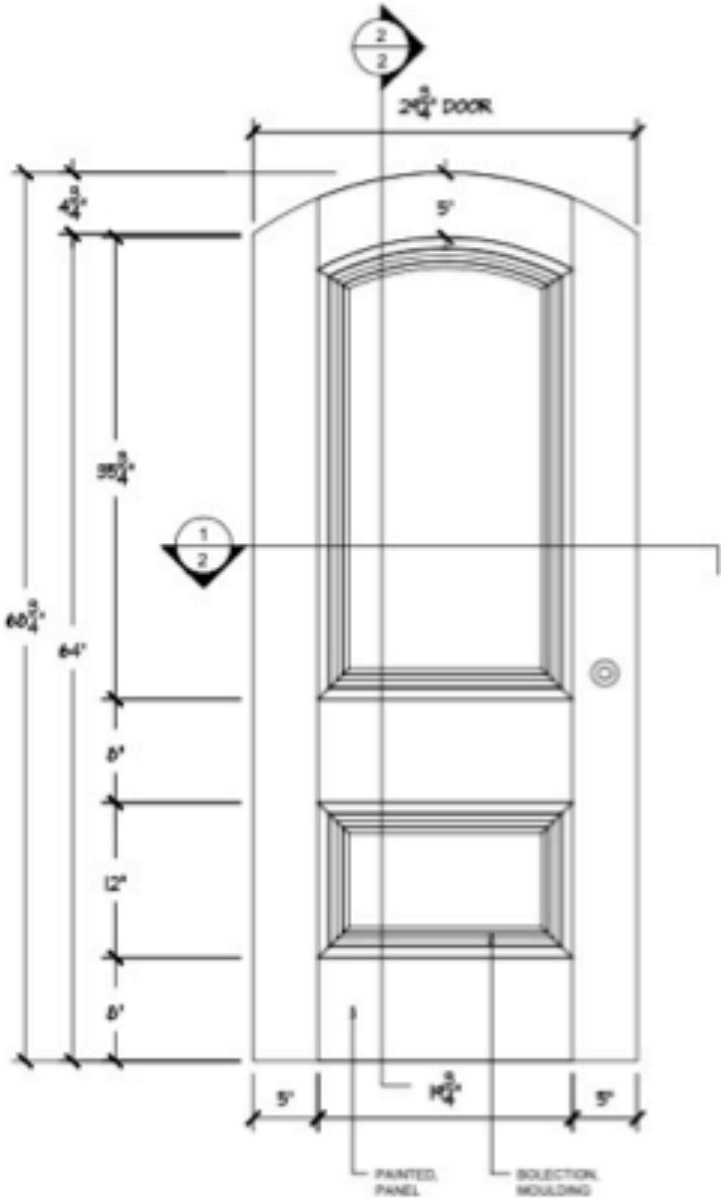
ELEVATION @ DOOR ARCH REF: 10/18 1/2" = 1'-0"
