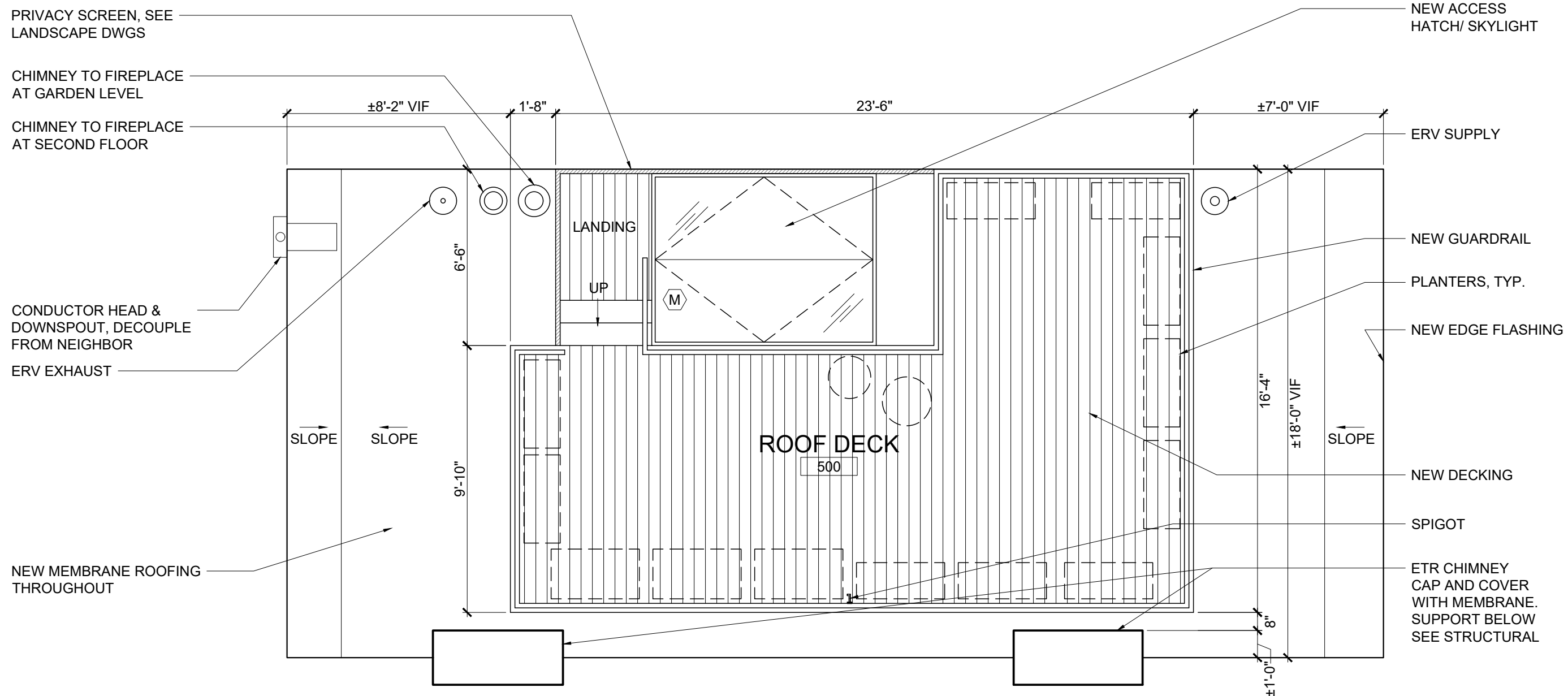
ROOF DECK LAYOUT
