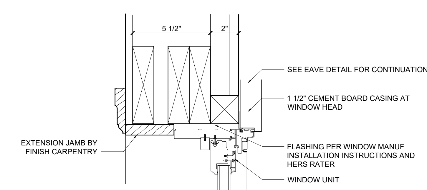
7 HEAD IN FRAMED OPENING 3"=1'-0"
