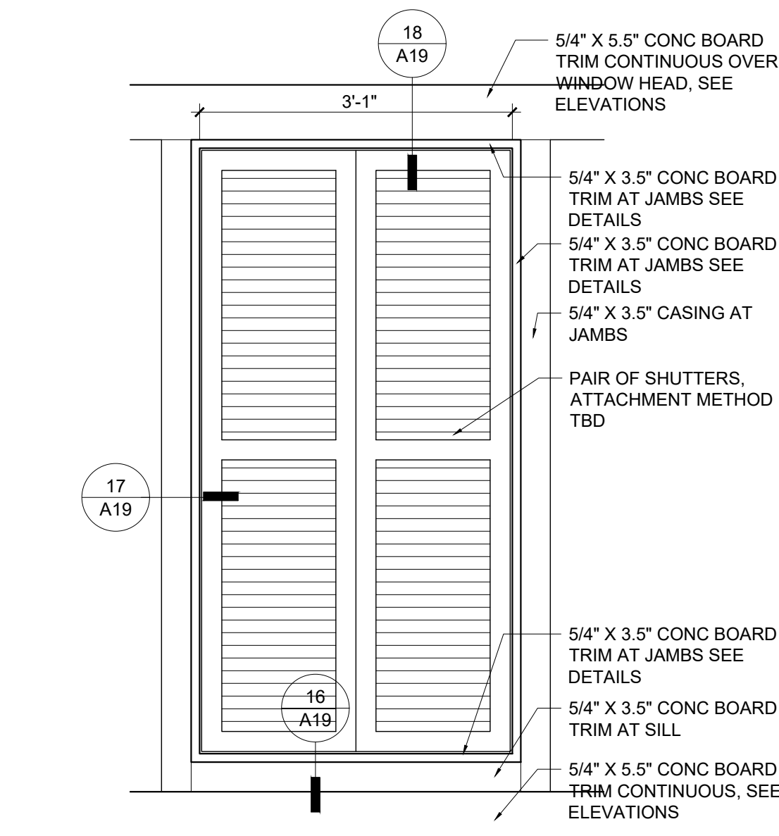
4 SHUTTER ELEVATION 3/4"=1'-0"
