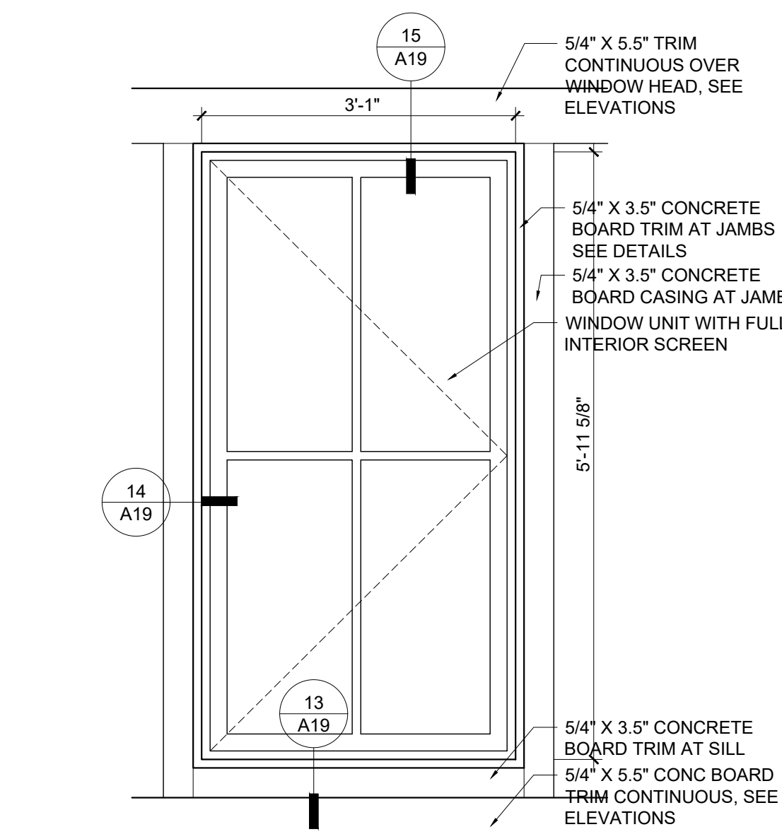
3 WINDOW TYPE O & N DETAIL ELEVATION 3/4"=1'-0"
