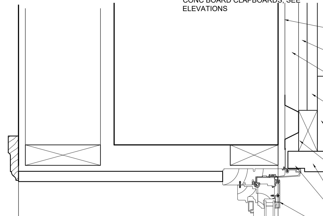
15 HEAD AT TYPE N & O 3"=1'-0"
