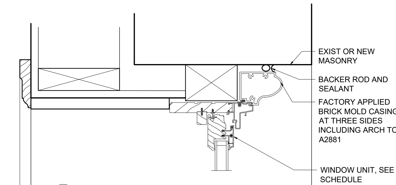
11 HEAD AT MO - CURVED & FLAT 3"=1'-0"
