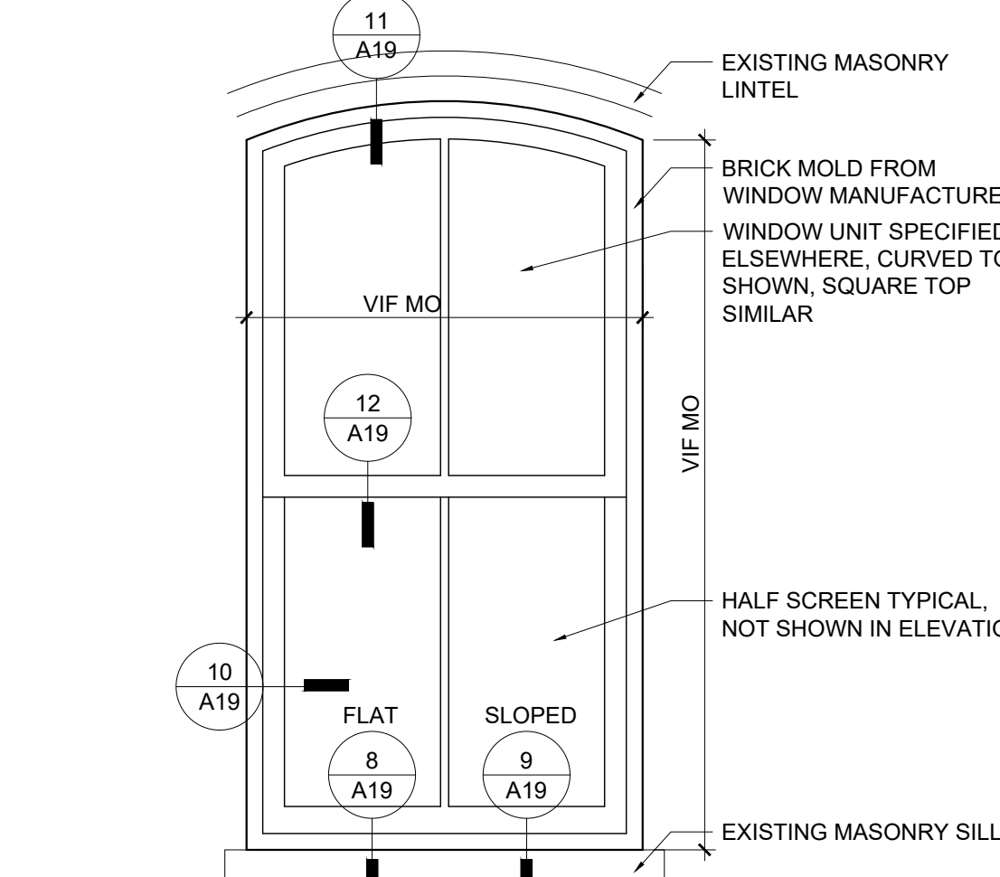
2 SQUARE & ARCH TOP WINDOWS IN MASONRY OPENING 3/4"=1'-0"
