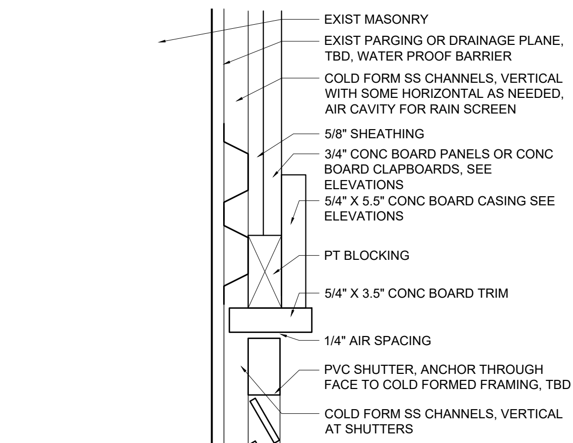
18 SHUTTER HEAD 3"=1'-0"
