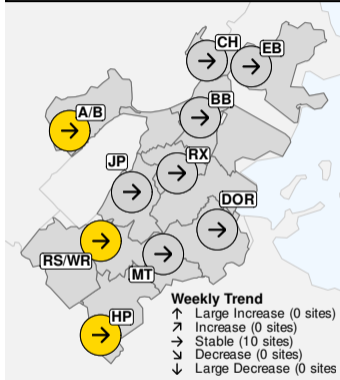
Influenza Wastewater Viral Activity Levels & Trends (28-Jun-2026)
