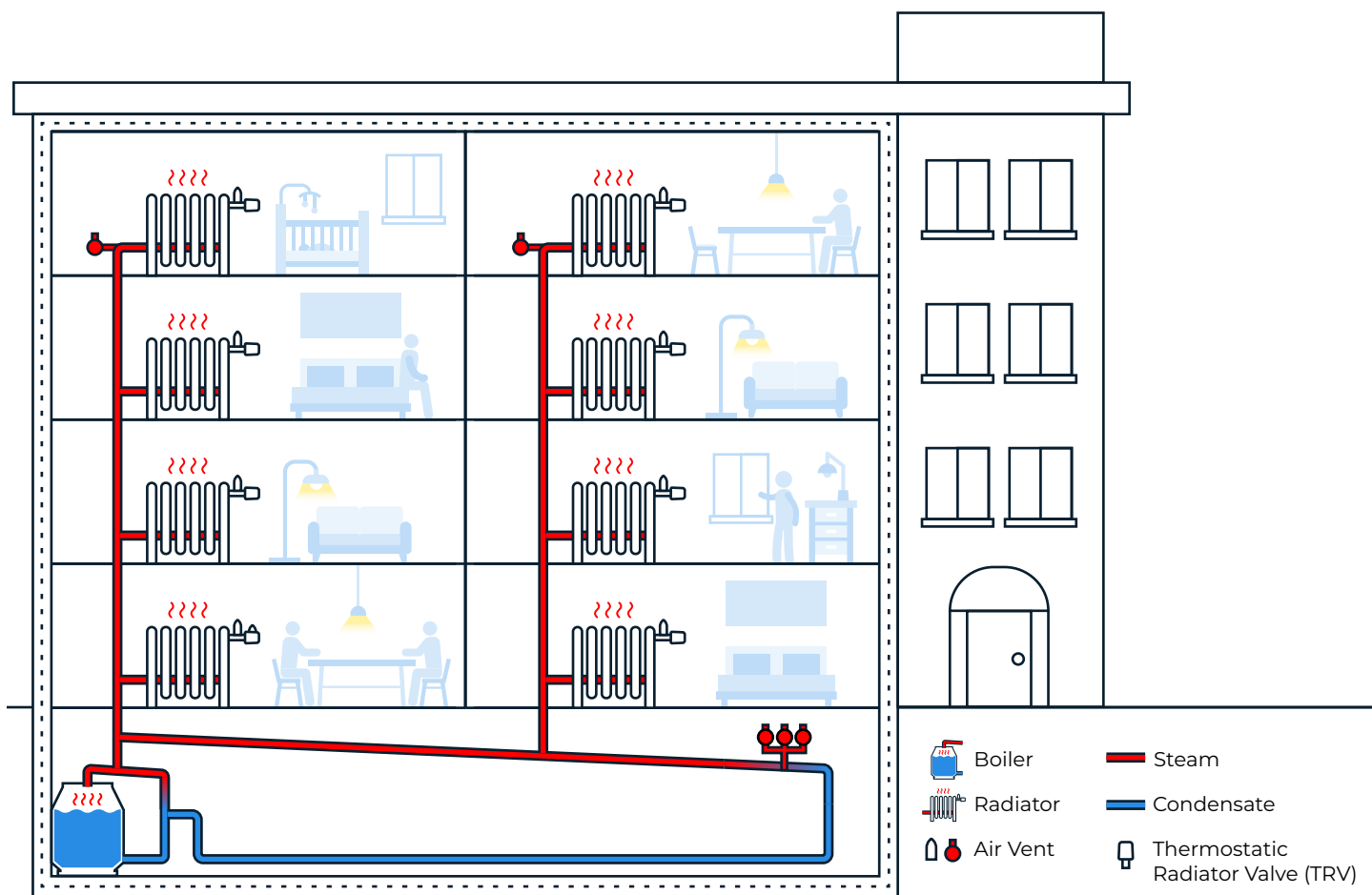
Optimized one-pipe steam system in a mid-rise multifamily building
