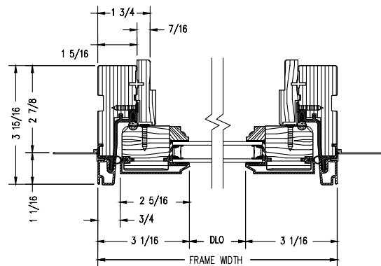
Horizontal Section
