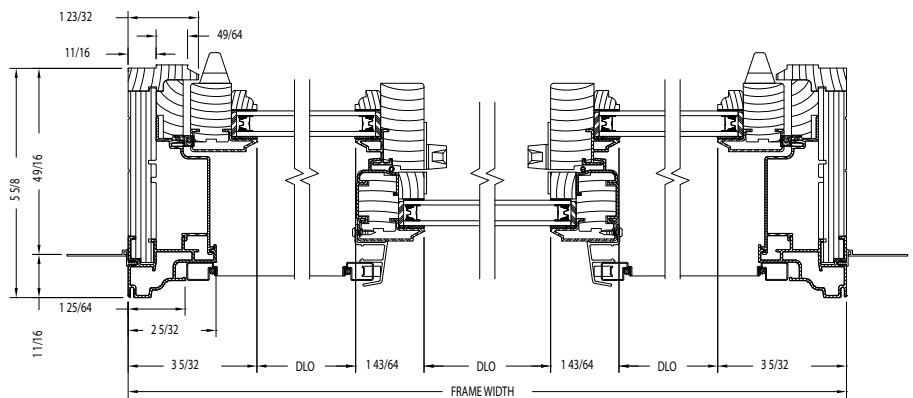
Horizontal Section
