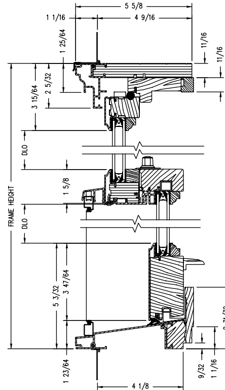
Vertical Section
